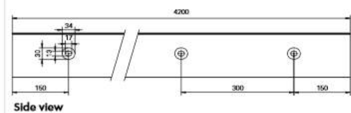
Face mount pre-machined hole positions
