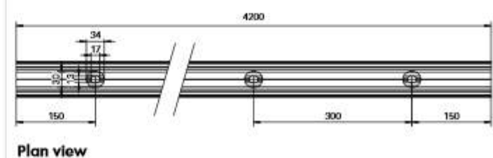
Deck mount pre-machined hole positions
